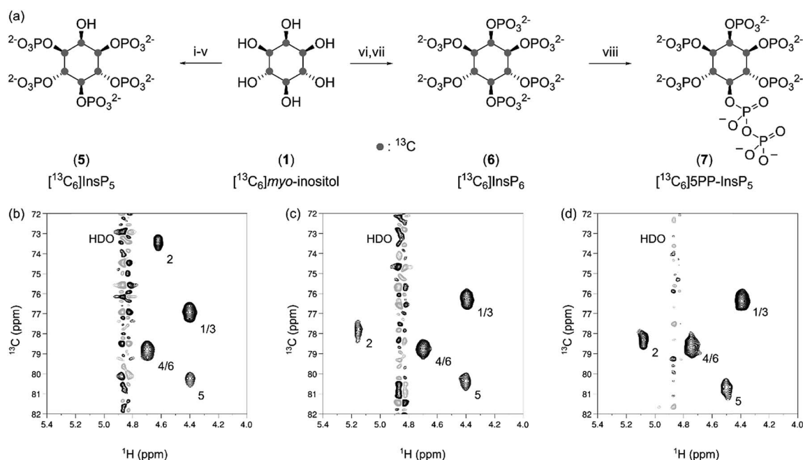
Fig. 3 Synthesis and characterization of ^{13}\text{C}_6 inositol polyphosphates. (a) Reagents and conditions: (i) CSA, trimethyl orthobenzoate, TEA in DMSO at 80 °C; 85% yield (ii) TFA in \text{H}_2\text{O} at rt; quantitative yield (iii) 5-phenyltetrazole, xylol phosphoramidite, mCPBA in DCM at rt; 79% yield (iv) \text{Pd}(\text{OH})_2/\text{C} in MeOH/ \text{H}_2\text{O} at rt; 88% yield (v) \text{NH}_3 (aq.) at 60 °C; 65% yield (vi) xylol phosphoramidite, 1H-tetrazole, mCPBA in DCM at rt; 38% yield (vii) \text{Pd}(\text{OH})_2/\text{C} in MeOH/ \text{H}_2\text{O} at rt; 83% yield (viii) MES pH 6.4, NaCl, ATP, creatine phosphate, \text{MgCl}_2 , DTT, IP6KA in \text{H}_2\text{O} at 37 °C; quantitative yield (b) ^1\text{H} , ^{13}\text{C} -HMQC spectrum of ^{13}\text{C}_6 InsP 5 at 5 \mu\text{M} . (c) ^1\text{H} , ^{13}\text{C} -HMQC spectrum of ^{13}\text{C}_6 InsP 6 at 5 \mu\text{M} . (d) ^1\text{H} , ^{13}\text{C} -HMQC spectrum of ^{13}\text{C}_6 5PP-InsP 5 at 5 \mu\text{M} . The positions of the carbon atoms and the solvent signal are indicated.
