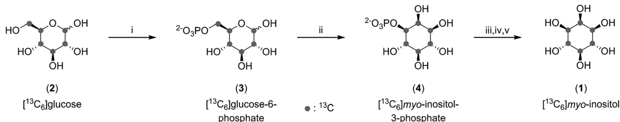
Fig. 2 Enzymatic synthesis of ^{13}\text{C}_6 myo-inositol followed by derivatization and purification. (i) MOPS pH 6.5, creatine phosphate, ATP, DTT, \text{MgCl}_2 , hexokinase, creatine kinase in \text{H}_2\text{O} at rt. (ii) Tris pH 8.0, \text{NAD}^+ , NaCl, \text{MgCl}_2 , inositol phosphate synthase in \text{H}_2\text{O} at 80 °C. (iii) Glycine pH 9.8, \text{ZnCl}_2 , alkaline phosphatase in \text{H}_2\text{O} at 35 °C. (iv) \text{Ac}_2\text{O} in pyridine at 120 °C. (v) NaOMe in MeOH at rt.
