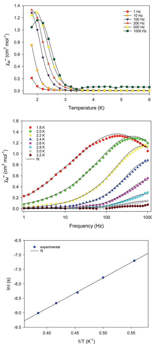
Fig. 4 (top) Out-of-phase ( \chi_M'' ) ac magnetic susceptibility signals for 1-w at zero dc field; the solid lines are guides for the eye. (middle) Frequency dependence of \chi_M'' at different temperatures for 1-w at zero dc field; the solid lines are best fits to the generalized Debye model. (bottom) Arrhenius plot of \tau versus 1/T for 1-w ; the solid line is the best fit as described in the text.
