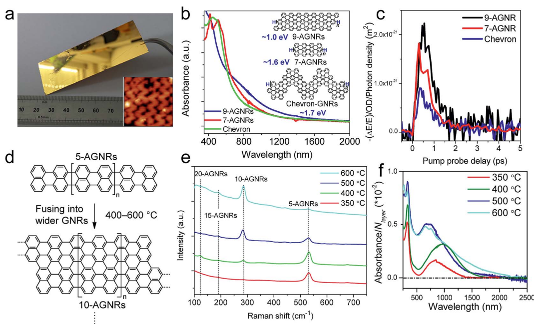
Fig. 5 On-surface synthesis of GNRs by CVD. (a) Photograph of a 25 \times 75 mm 2 Au/mica plate on which a GNR film could be grown. Inset shows the STM image of chevron-type GNRs. Reproduced with permission. 66 Copyright (2016) American Chemical Society. (b) UV-vis-NIR absorption spectra of different CVD-grown GNRs. The inset shows the chemical structures of the GNRs and their optical bandgaps. (c) Comparative study of THz photoconductivity of different GNR structures. (b and c) Reprinted with permission. 115 Copyright (2017) American Chemical Society. (d) Lateral fusion of 5-AGNR to form wider GNRs. (e) Raman spectra of extended AGNRs annealed at different temperatures showing the RBLM peaks of various GNRs of different widths. (f) UV-vis-NIR absorption spectra of AGNRs annealed at different temperatures. The spectra are normalized to the number of GNR layers ( N_{\text{layer}} ). (d–f) Reprinted with permission. 116 Copyright (2017) American Chemical Society.
