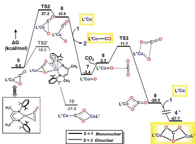
Fig. 6 M06L/def2-TZVPP Gibbs free energy ( \Delta G ) profile for the mononuclear dissociative pathway. Isolated species are shown in yellow boxes, with L' depicted instead of L' tu . *Marked species has lower relative free energy on the S = 3 surface which has been taken to complete the profile.
