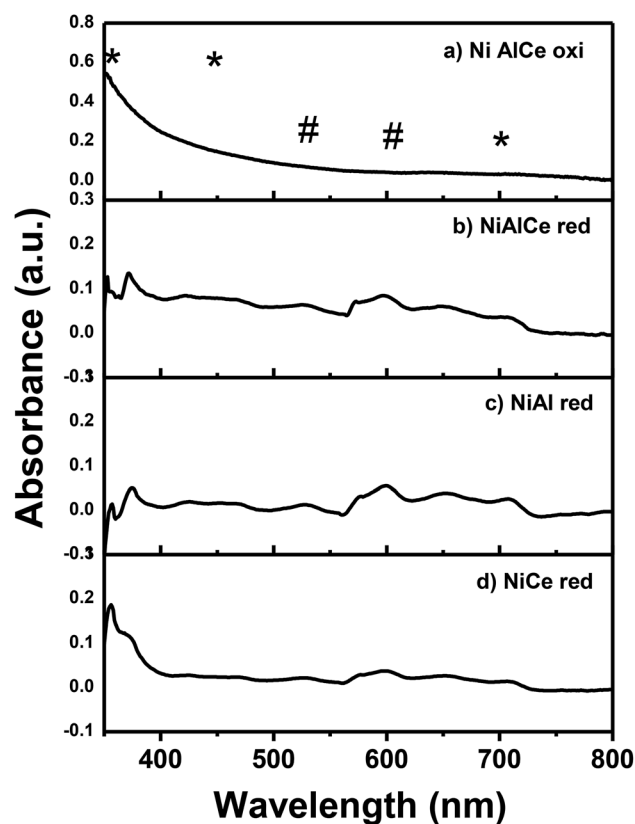
Fig. 6 Spectra UV-Vis for the calcined Ni supported catalyst: (a) and for the reduced Ni supported catalysts: (b), (c) and (d). Legend: (#) \text{Ni}^{+2} (Td), (*) \text{Ni}^{+2}(\text{OH}) .
