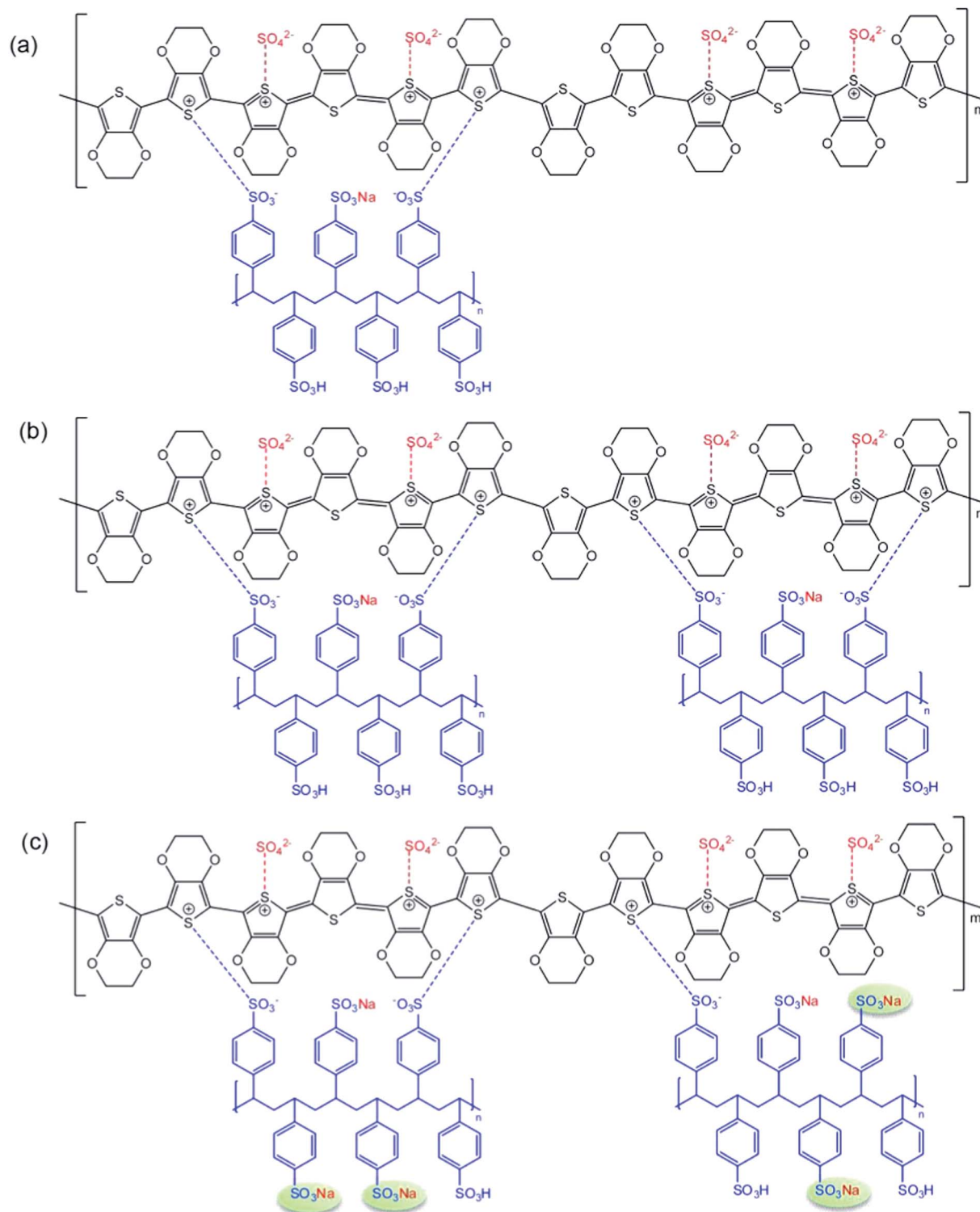
Scheme 2 Proposed interaction of PEDOT:PSS at the EDOT : Na_2S_2O_8 mole ratio of 1 : 1 and various EDOT : PSS weight ratios: at an EDOT : PSS weight ratio (a) lower than 1 : 11, (b) 1 : 11, where more PSS interact, and (c) higher than 1 : 11 with a higher PSSNa amount to reduce the doping sites on PSS.
