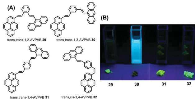
Fig. 19 Structures and fluorescence images of 29–32 in CH 2 Cl 2 solution (upper) and as solids (lower) (from left to right) under illumination by a 365.0 nm UV lamp.
