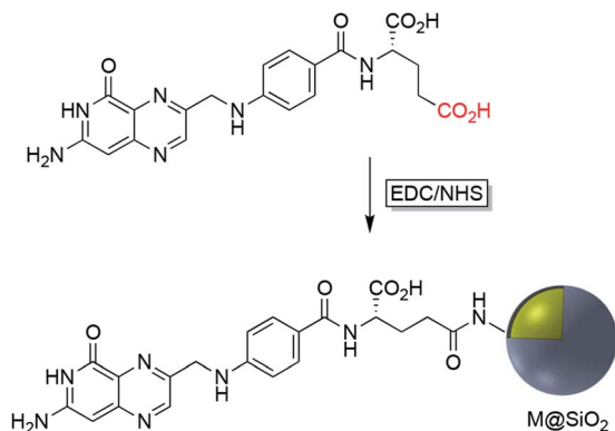
Fig. 6 Synthesis route to folic acid-conjugated silica-coated plasmonic nanoparticles (M = Ag, Au).
