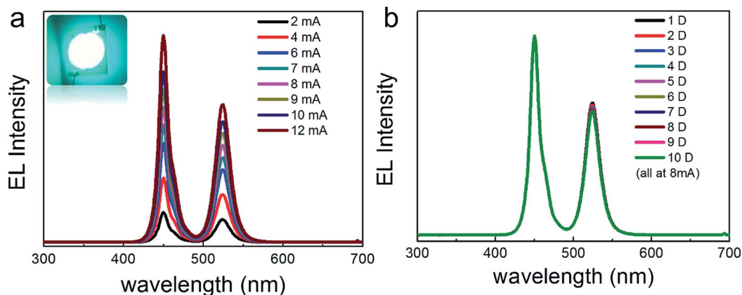
Fig. 9 (a) EL spectra of the \text{CsPbBr}_3@\text{Cs}_4\text{PbBr}_6 NC powder-based backlit LED under different currents; inset is the photograph of the backlit LED. (b) EL spectra of the \text{CsPbBr}_3@\text{Cs}_4\text{PbBr}_6 -based backlit LED lighted for 10 days under ambient conditions.
