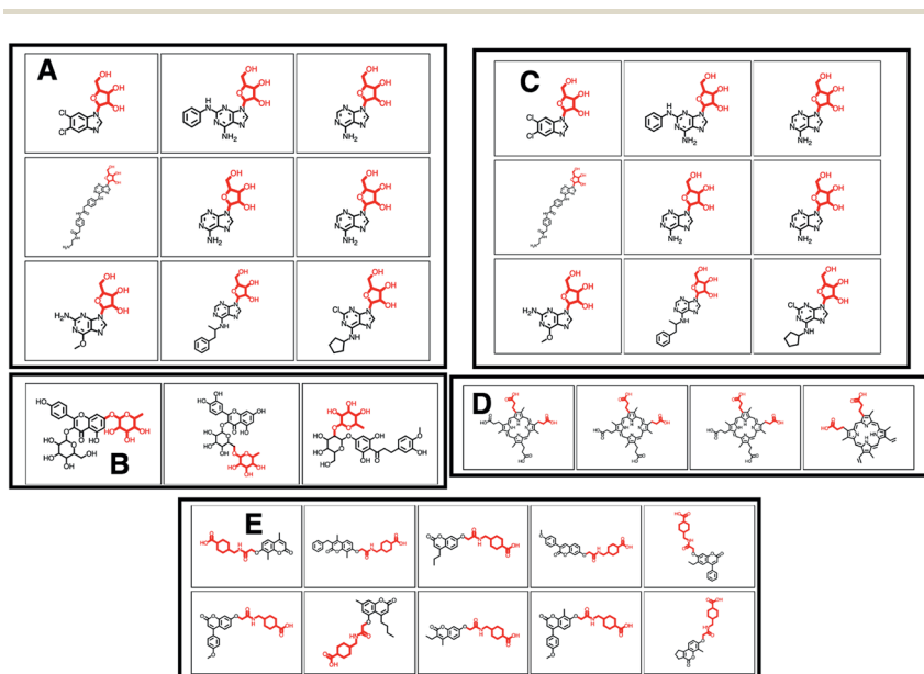
Fig. 3 (A–E) Screenshots of the ms2lda.org web app with (A) 9 different molecules out of the 50 molecules that MAGMa annotated with a hexose moiety for the loss feature in MassBank Mass2Motif 41. (B) 3 examples of the 13 molecules where MAGMa annotated the loss feature in MassBank Mass2Motif 41 with a deoxyhexose moiety. (C) 9 out of the 27 molecules for which MAGMa annotated a pentose moiety for the loss feature in GNPS Mass2Motif 44. (D) Alternative loss annotation of the loss feature in GNPS Mass2Motif 44. (E) Oxyacetyl-amino-methyl-cyclohexane-1-carboxylic acid loss annotated in 10 molecules of GNPS Mass2Motif 439.
