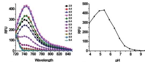
Fig. 52 Acid-activatable fluorescence of probe 36 . A series of phosphate buffer solutions (pH 3.9–9.4) containing 36 ( 200 \mu\text{M} ) was analyzed for fluorescence emission using an excitation wavelength of 715 \text{ nm} . Copyright 2015 American Chemical Society.
