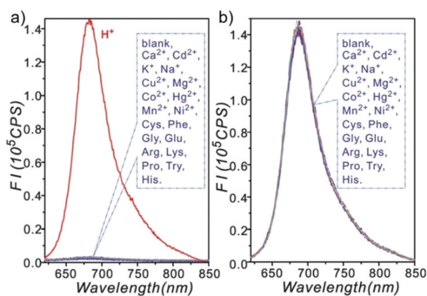
Fig. 39 Fluorescence responses of 26a (10 \mu\text{M} ) to different analytes; K^+ (100 mM), Na^+ (100 mM), Ca^{2+} (0.5 mM), Cd^{2+} (0.3 mM), Cu^{2+} (0.3 mM), Mg^{2+} (0.5 mM), Co^{2+} (0.3 mM), Hg^{2+} (0.3 mM), Mn^{2+} (0.3 mM), Ni^{2+} (0.3 mM), Cys (0.1 mM), Phe (0.1 mM), Gly (0.1 mM), Glu (0.1 mM), Arg (0.1 mM), Lys (0.1 mM), Pro (0.1 mM), Try (0.1 mM) and His (0.1 mM) were included. (a) Tested in disodium hydrogen phosphate-citric acid buffer (pH 7.0). (b) Tested in citric acid buffer (pH 1.6). Copyright 2013 Royal Society of Chemistry.
