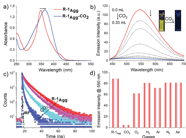
Fig. 2 (a) Absorption spectra of R-1 ( 1 \times 10^{-4} M) in aqueous medium (water/DMSO, 99/1 v/v) after purging with excess amount of \text{CO}_2 (0.33 mL). (b) Emission spectra of R-1 ( 1 \times 10^{-4} M, \lambda_{\text{ex}} = 370 nm) in the presence of different concentrations of \text{CO}_2 (0, 0.016, 0.032, 0.048, 0.064, 0.080, 0.096, and 0.33 mL). Inset shows the fluorescence change of R-1 under UV illumination ( \lambda_{\text{ex}} = 365 nm) before and after purging with \text{CO}_2 . (c) Fluorescence lifetime decay profile of R-1 ( \lambda_{\text{ex}} = 370 nm, \lambda_{\text{em}} = 550 nm) in the presence of increasing \text{CO}_2 concentrations (0, 0.016, 0.048 and 0.33 mL). IRF = instrument response function. (d) Fluorescence response ( \lambda_{\text{ex}} = 370 nm) of R-1 towards \text{CO}_2 after purging with different gases (3.0 mL) in aqueous medium; from left to right: R-1 , \text{CO}_2 , \text{O}_2 , \text{H}_2 , Ar, \text{N}_2 and air.
