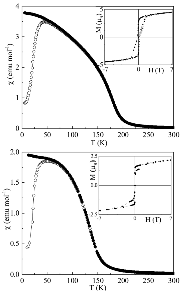
Fig. 2 Magnetic susceptibilities of \text{CaMnCoReO}_6 (top) and \text{CaMnNiReO}_6 (bottom) with insets showing magnetization-field loops at 7 and 2 K respectively.
