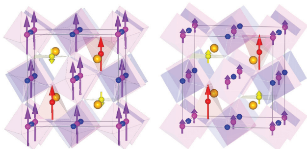
Fig. 3 Crystal and magnetic structures of \text{CaMnCoReO}_6 (left) and \text{CaMnNiReO}_6 (right) with the z -axis vertical. Orange, red, yellow, purple and blue spheres represent Ca, A' , A'' , B and Re sites respectively. Polyhedra show the tetrahedral, square planar and octahedral coordination of A' , A'' and B sites, and arrows show the spin directions scaled to the refined magnitudes of the ordered moments.
