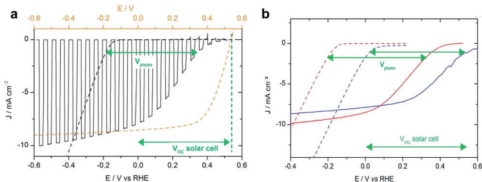
Fig. 4 (a) Voltammogram recorded at 50 \text{ mV s}^{-1} in 0.5 \text{ M H}_2\text{SO}_4 with chopped visible light for an ITO/PEDOT:PSS/P3HT:PCBM/LiF/Al/Ti-Mo \text{S}_3 photocathode (black line, electrode area 0.32 \text{ cm}^2 ) and recorded at 5 \text{ mV s}^{-1} in 0.5 \text{ M H}_2\text{SO}_4 for an ITO-Mo \text{S}_3 cathode (black dashed line, electrode area 0.28 \text{ cm}^2 ). Potentials are referred to the RHE (bottom axis). The current-voltage curve of an ITO/PEDOT:PSS/P3HT:PCBM/LiF/Al solar cell (orange dashed line, top axis) is shown for comparison. (b) Voltammogram recorded at 5 \text{ mV s}^{-1} in 0.5 \text{ M H}_2\text{SO}_4 for an ITO-Mo \text{S}_3 cathode (red dotted line) and an ITO-Pt/C cathode (blue dotted line) and at 50 \text{ mV s}^{-1} with visible-light illumination ( 100 \text{ mW cm}^{-2} ) for an ITO/PEDOT:PSS/P3HT:PCBM/LiF/Al/Ti-Mo \text{S}_3 photocathode (red line) and an ITO/PEDOT:PSS/P3HT:PCBM/LiF/Al/Ti-Pt/C photocathode (blue line). Reprinted with permission from Bourgeteau, et al. , ACS Appl. Mater. Interfaces , 7, 30, 16395–16403. Copyright (2015) American Chemical Society. 31
