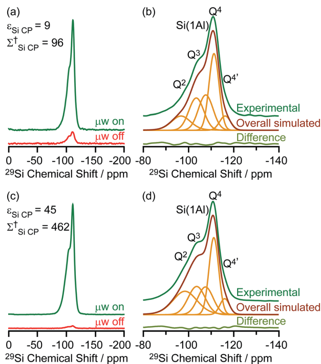
Fig. 6 (a and c) 29 Si CP MAS DNP spectra and (b and d) \mu\text{w} on experimental 29 Si CP MAS DNP spectra with spectral deconvolution, overall simulated lineshape and difference between experimental and simulated spectra of activated M-β (a and b) and activated MMM-β (c and d). All spectra were recorded at 9.4 T and at a MAS rate of 8 kHz. \Sigma^{\dagger} refers to the overall DNP gain and is calculated by comparing the DNP data to room temperature 9.4 T NMR spectra (see ESI†).
