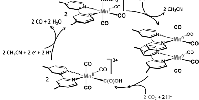
Scheme 6 The catalytic cycle for two-electron reduction of CO 2 to CO with [Mn(bpy)(CO) 3 ] + . Reprinted with permission from ref. 113. Copyright 2014, WILEY-VCH Verlag GmbH.
