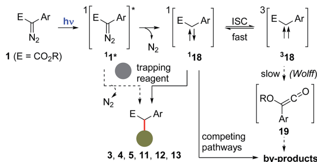
Scheme 9 Proposed mechanistic scenario involved in the formation of the products 3 , 4 , 5 , ^1\mathbf{11} , ^1\mathbf{12} and ^1\mathbf{13} , and plausible explanations for the formation of by-products.
