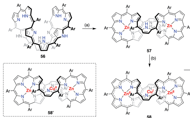
Fig. 18 Synthesis of the decaphyrin Zn(II)–Cu(I)–Zn(II) complex 58 . (a) 5 equiv. Zn(OAc)_2 \cdot 2H_2O , 5 equiv. NaOAc, MeOH, reflux, 2 h, 61%; (b) 10 equiv. Cu(OAc)_2 , 10 equiv. NaOAc, MeOH, rt, 4 h, 72%. Ar = pentafluorophenyl.
