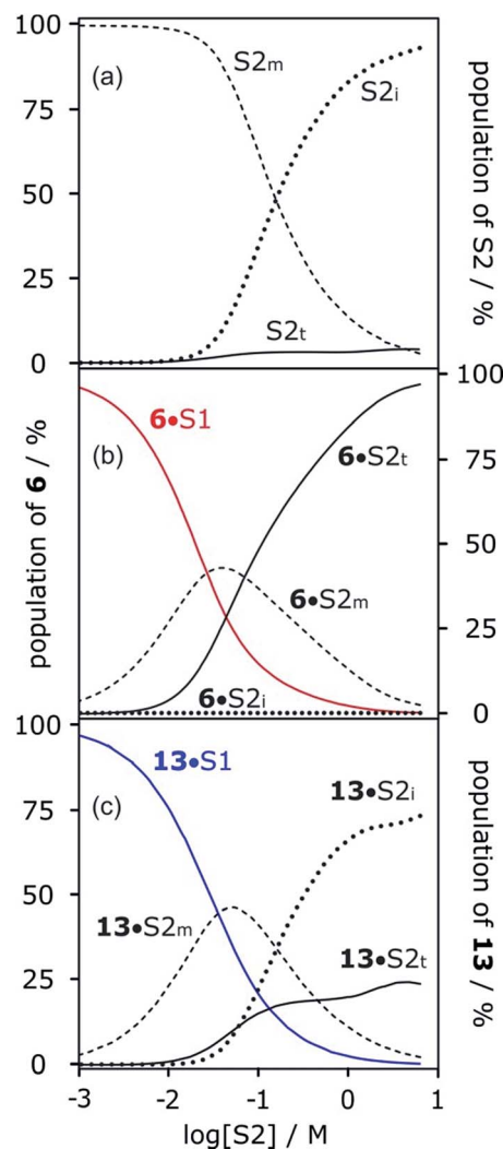
Fig. 12 (a) Speciation of alcohol monomer ( S2_m ), internal ( S2_i ) and terminal ( S2_t ) H-bonding sites in mixtures of 1-octanol (S2) and n -octane (S1). (b) Speciation of solvation states of H-bond acceptor solute 6 in mixtures of 1-octanol (S2) and n -octane (S1): 6 ·S1 solid red line; 6 · S2_m dashed line; 6 · S2_i dotted line; 6 · S2_t solid black line. (c) Speciation of solvation states of H-bond donor solute 13 in mixtures of 1-octanol (S2) and n -octane (S1): 13 ·S1 solid blue line; 13 · S2_m dashed line; 13 · S2_i dotted line; 13 · S2_t solid black line. Calculated using the following H-bond parameters for S2: \alpha_i = 0 , \alpha_t = 3.5 , \alpha_m = 2.7 and \beta_i = 5.3 , \beta_t = 6.9 , \beta_m = 5.3 .
