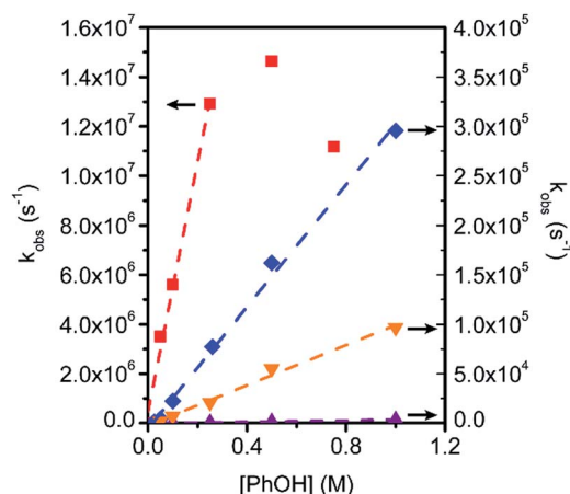
Fig. 4 Observed rate constants ( \text{s}^{-1} ) for catalytic CO 2 reduction as a function of PhOH concentration for Fe- ortho -1-amide (blue diamonds), Fe- ortho -2-amide (red squares), Fe- para -1-amide (purple upward triangles), and Fe- para -2-amide (orange downward triangles). Conditions: 1 mM catalyst, 0.1 M TBAPF 6 in DMF; 0.23 M CO 2 ; scan rate is 100 mV s -1 . k_{\text{obs}} values were determined by FOWA.
