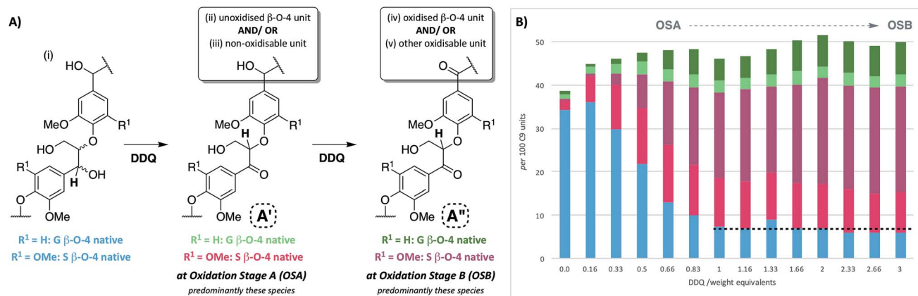
Fig. 3 Beech lignin DDQ oxidation study: (A) proposed reactivity of β-O-4 units within lignin including possible oxidized stages within lignin ^{\alpha-ox} of the β-O-4 unit. The chemical shifts of the highlighted H atoms are reliant on the substituents on the aromatic ring connected via the aryl-ether linkage (Fig. S1†); (B) graph displaying β-O-4 and β-O-4 ^{\alpha-ox} units per 100 C9 units against DDQ weight equivalents; highlighted H atoms (and their corresponding cross-peaks within 2D HSQC analysis) were used for semi-quantification of units within lignin. 38 Data repeated in triplicate, for standard error analysis, see Table S3.† All standard errors associated with values in this figure are <1.5%. *Dashed lines indicate a plateau where no more oxidation was notably occurring. No/very little signal corresponding to remaining β-O-4 native units were observed at this point in 2D HSQC NMR spectra, but background noise and/or new peaks may be overlapping with integral regions rendering these integrals not equal to zero.
