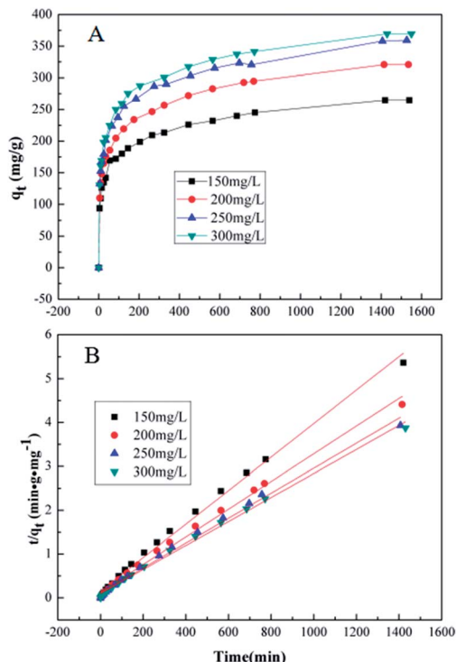
Fig. 7 (A) The adsorption capacity of GMFP nano-composites for different concentrations of Cr(vi) ions with time. (B) The pseudo-second-order model for adsorption of Cr(vi) ions by GMFP nanocomposites.
