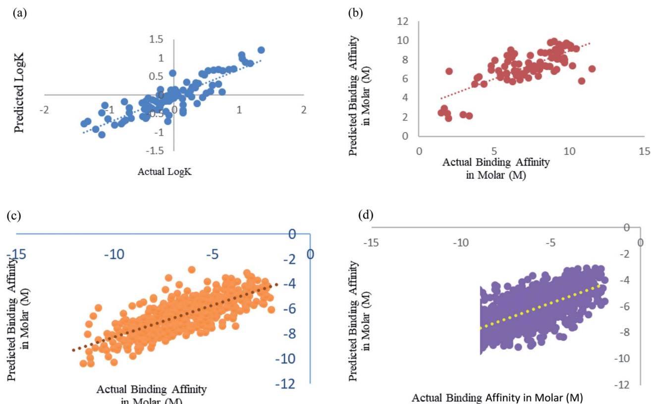
Fig. 5 (a) Scatter plot for actual vs. predicted log K of Xue's dataset using SMO utilising RBF kernel over 10-fold cross-validation. (b) Scatter plot for actual vs. predicted binding affinity of Deng's dataset using Random forest over 10-fold cross validation. (c) Scatter plot for actual vs. predicted binding affinity of Wang's dataset using Random forest. (d) Scatter plot for actual vs. predicted binding affinity of Kramer's dataset using Random forest.
