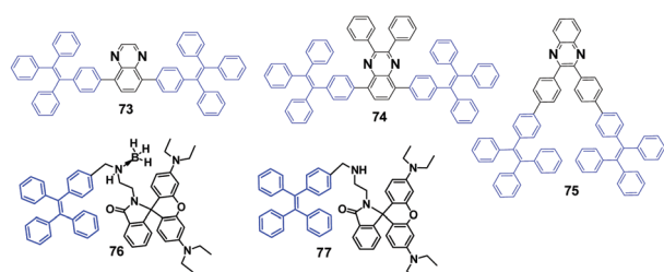
Fig. 21 The molecular structures of compounds 73–75 .
