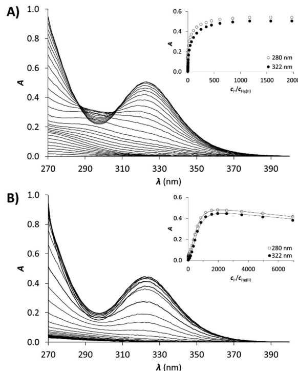
Fig. 5 UV spectra recorded in the titration of (A) Hg(II) and (B) Hg 1 C with I − . pH = 2.0, C_{Hg(II)} = 30 μM (A), C_{Hg(II)} = C_{peptide} = 30 μM (B). The insets show the evolution of the absorbance at 322 nm (●) and 280 nm (○). Symbols represent the experimental data, and solid lines represent the absorbances calculated by SPECFIT.
