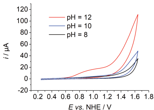
Fig. 2 pH dependent CV data of 1 in Millipore water ([ 1 ] \approx 1 mM, \nu = 0.1 M PO 4 3- , \nu = 0.1 mV s -1 ).
