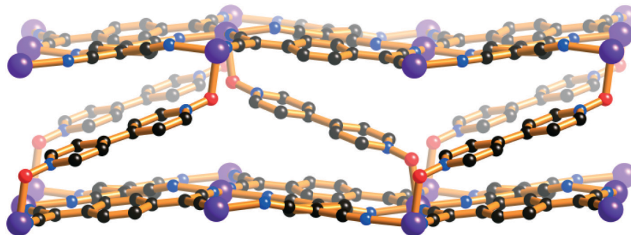
Fig. 8 The structure of [\text{Zn}(\text{TCNQ})(\text{Obip})_{1/2}(\text{MeOH})] ( 43 ). The Obip ligands are inclined with respect to the sheets to form close charge transfer interactions with the \text{TCNQ}^{2-} ligands. For clarity, the coordinated MeOH ligands have been omitted.
