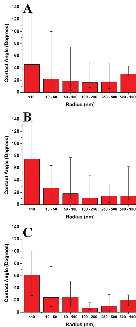
Fig. 14 Graphs showing the radius against contact angle for the nano-droplets on a mica surface at varying molecular weights. Each graph presents the average values and has bars which indicate the range of values. (A) M_n = 46 \text{ kg mol}^{-1} , (B) M_n = 86 \text{ kg mol}^{-1} , (C) M_n = 355 \text{ kg mol}^{-1} .
