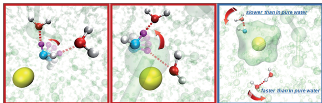
Fig. 1 The schematic representation of cation effects on the water rotation. Panels left and middle: the effect of a cation (yellow) on the jump motion of a water molecule. In the left panel, the jump of the water molecule (O labeled in cyan) between two H-bond acceptors (O labeled in red) is accelerated by the binding of the (Na + or K + ) cation. In the middle panel, the binding of the cation to one H-bond acceptor accelerates the jump of the water molecule (O labeled in cyan) switching between this acceptor and another (O labeled in red). The right panel illustrates the diffusive rotations of water pairs inside/outside the ion solvation shell (green). The average diffusive mobility of water is decided by the balance between these two contributions.
