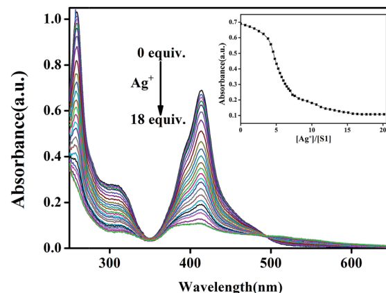
Fig. 4 Absorbance spectra of S1 ( 20 \mu\text{M} ) in the presence of different concentrations of \text{Ag}^+ (0–18 equiv.) in the DMSO/ \text{H}_2\text{O} (v:v = 1 : 1, buffered with HEPES pH = 7.2) solution. Inset: A plot of the variation in absorbance as a function of concentration of \text{Ag}^+ in the range from 0 to 18 equiv.
