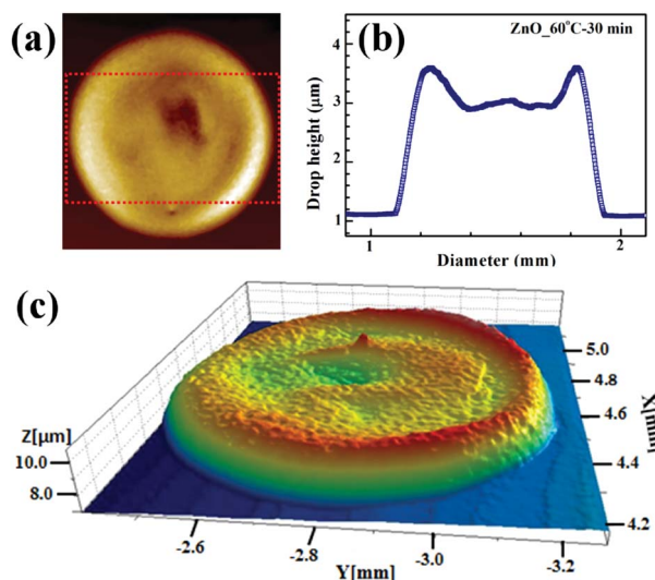
Fig. 12 ZnO drop dried at 60 °C for 30 min in hot air oven. (a) Optical image shows relatively crack-free surface, (b) line profile (from the red dotted region marked in (a)) shows uniform drying with some particle accumulation still seen at the edges. (c) This minor variation in thickness from the rim to the centre of drop can be seen clearly in the 3D image.
