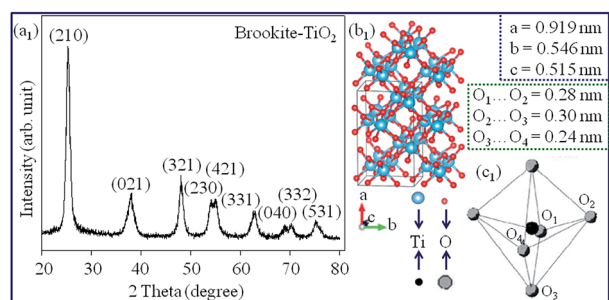
Fig. 8 Structural characteristics of brookite- \text{TiO}_2 : (a 1 ) XRD pattern, 275 (b 1 ) ball-and-stick structure, 142 (c 1 ) an orthorhombic crystalline struc- ture. 256 Colour code; O atoms: red (small balls), grey (large balls) and Ti atoms: blue (large balls), black (small balls). Unit cells are outlined using thin lines. (a 1 ) is reprinted with permission from ref. 275. Copyright 2015. VBRI Press. (b 1 ) is reprinted with permission from ref. 142. Copyright 2014. American Chemical Society. (c 1 ) is reprinted with permission from ref. 256.
