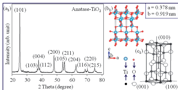
Fig. 7 Structural characteristics of anatase- \text{TiO}_2 : (a 1 ) XRD pattern, 275 (b 1 ) ball-and-stick structure, 142 (c 1 ) the tetragonal system with a dipyr- amidal habit. 256 Colour code; O atoms: red (small balls), grey (large balls) and Ti atoms: blue (large balls), black (small balls). Unit cells are outlined using thin lines. (a 1 ) is reprinted with permission from ref. 275. Copyright 2015. VBRI Press. (b 1 ) is reprinted with permission from ref. 142. Copyright 2014. American Chemical Society. (c 1 ) is reprinted with permission from ref. 256.
