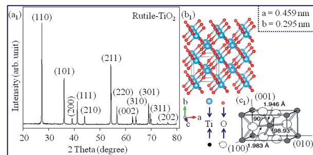
Fig. 9 Structural characteristics of rutile- \text{TiO}_2 : (a 1 ) XRD pattern, 23 (b 1 ) ball-and-stick structure, 142 (c 1 ) the tetragonal system with a prismatic habit. 256 Colour code; O atoms: red (small balls), grey (large balls) and Ti atoms: blue (large balls), black (small balls). Unit cells are outlined using thin lines. (a 1 ) is reprinted with permission from ref. 23. Copyright 2016. Elsevier. (b 1 ) is reprinted with permission from ref. 142. Copyright 2014. American Chemical Society. (c 1 ) is reprinted with permission from ref. 256.
