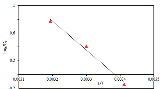
Fig. 11 Plot of \ln(q_e/C_e) versus 1/T for the adsorption of Cr(vi) on SMGO. Mass of SMGO = 0.5 \text{ g L}^{-1} , initial concentration of Cr(vi) = 100 \text{ mg L}^{-1} , contact time = 60 min, \text{pH} = 3 , volume of Cr(vi) = 40 mL.
