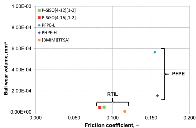
Fig. 4 Ball wear volume versus mean friction coefficient as determined by initial screening test under conditions C\{100\text{ N}/25\text{ }^\circ\text{C}/60\text{ min}\} . The RTILs provide better lubrication, resulting in lower friction and wear compared to the evaluated PFPEs.
