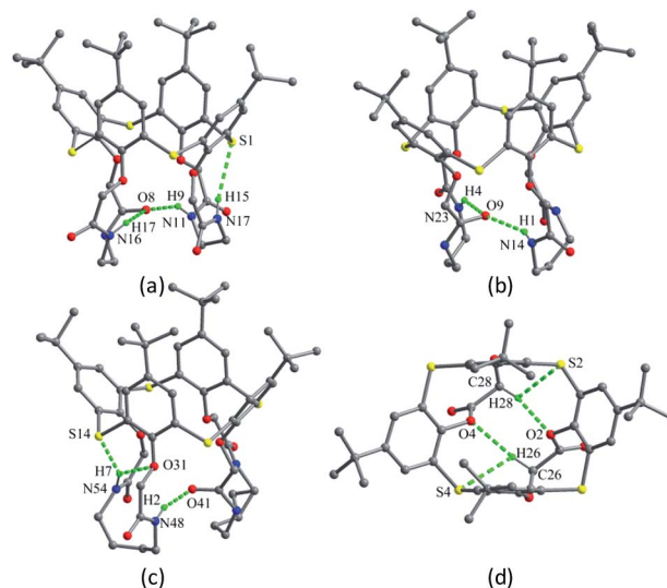
Fig. 33 Crystal structures of 40 (a), 41 (b), 42 (c) and 43 (d), showing intramolecular H-bonds.
