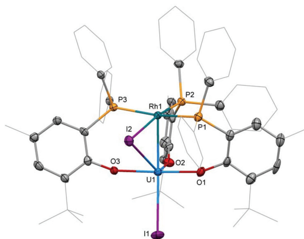
Fig. 2 Molecular structure of 3 . Solvent molecules and hydrogen atoms are omitted and peripheral carbon atoms are depicted as wire-frame for clarity. Thermal ellipsoids drawn at 50% probability. Selected distances (Å) and angles (°): U1–Rh1: 2.7630(5), U1–I1: 3.0428(5), U1–I2: 3.2264(5), U–O: 2.129(4)–2.156(3), Rh1–I2: 2.7296(6), Rh–P: 2.318(1)–2.416(1), I1–U1–Rh1: 167.75(2), U1–I2–Rh1: 54.51(1).
