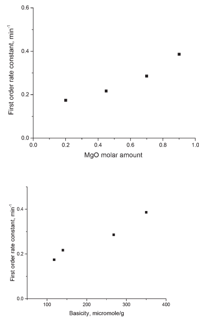
Fig. 9 Galactose isomerization first order rate constant vs. a) molar Mg content and b) basicity of magnesium aluminates. Reaction conditions: 110 °C, m_{\text{cat}} = 9.2 g, 5 bar, 1000 rpm and calcination temperature = 680 °C.
