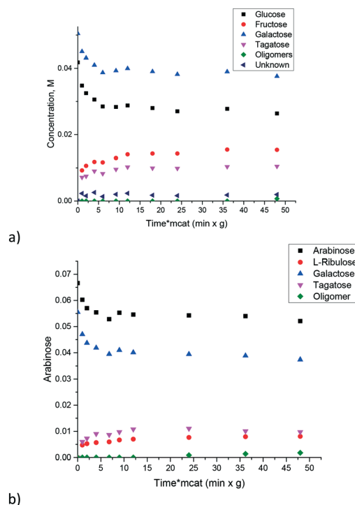
Fig. 10 Isomerization of sugar mixtures over the (MgO) 0.8 (Al 2 O 3 ) 0.2 catalyst for a) galactose–glucose and b) galactose–arabinose mixtures. Reaction conditions: temperature = 110 °C, calcination temperature = 680 °C, m_{\text{cat}} = 0.2 g, 5 bar and 1000 rpm.
