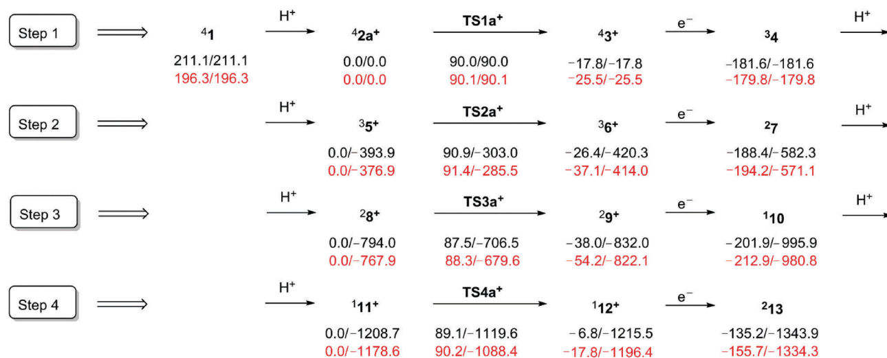
Scheme 3 Energetics of the four-step synthesis of NH_4^+@C_{60}^{*-} 13 via the most favorable transition states and spin states. Energies in \text{kcal mol}^{-1} within a step vs. (/) relative to 42a^+ at the B3LYP (black) and at the MP2 (red).
