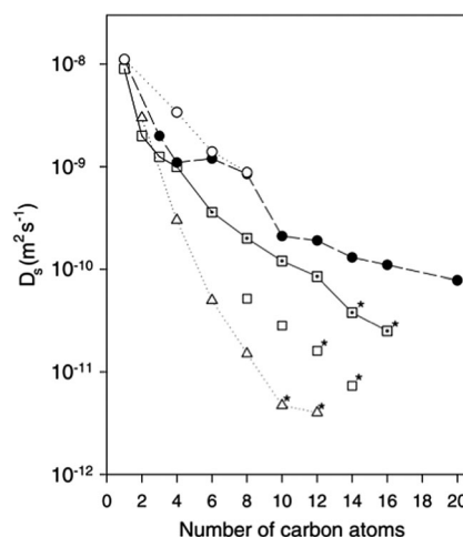
Fig. 2 Self-diffusivities obtained at 300 K from MD simulations ( \circ ), 35 hierarchical simulations ( \bullet ), 50 QENS in Na-ZSM-5 ( \square ), 46 QENS in silicalite-1 ( \nabla ) 47 and PFG-NMR ( \Delta ). 49 * = extrapolation to 300 K. Figure reproduced from ref. 47 with permission from the American Chemical Society.
