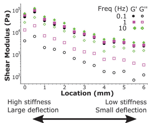
Fig. 7 Mapping viscoelastic properties over a large stiffness range on a HS–LS gradient sample. At a high stiffness location (left) the large cantilever deflection ( \sim 20\ \mu\text{m} ) can be measured while at a low stiffness location (right) the small cantilever deflection ( \sim 200\ \text{nm} ) can also still accurately quantify stiffness. At a controlled indentation depth the material is deformed to the same degree on all locations, while the viscoelasticity is quantified over more than one order of magnitude.
