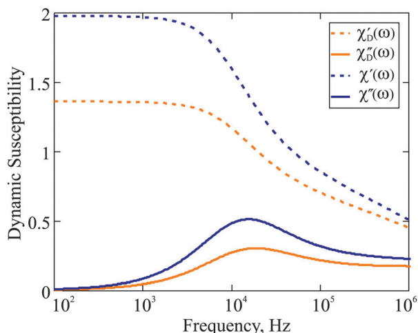
Fig. 1 Dynamic susceptibility 4\pi\chi(\omega) of comparison of the Debye ideal gas model to the expressions in eqn (18). The frequency range is given on the log-scale. Here, \phi_m = 0.06 ; T = 293 K; K = 20 kJ m ^{-3} ; effective viscosity \eta = 2 \times 10^{-3} Pa s; M_0 = 480 kA m ^{-1} .
