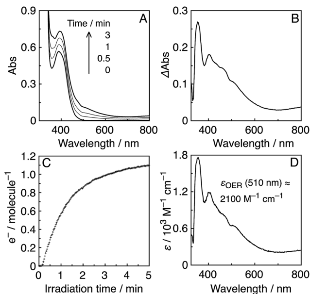
Fig. 4 (A) UV-vis absorption spectral changes of an Ar-saturated DMF–TEOA (5 : 1 v/v) solution containing R(5) (0.05 mM) under irradiation at \lambda_{ex} = 436 nm ( 5.6 \times 10^{-9} einstein per s). (B) Differential absorption spectrum before irradiation and after 3 min irradiation. (C) Time course of accumulated electrons in R(5), compensated for the inner filter effect. (D) Differential absorption spectrum of R(5) before and after bulk electrolysis in an Ar-saturated DMF solution at -1.95 V vs. Ag/AgNO 3 .
