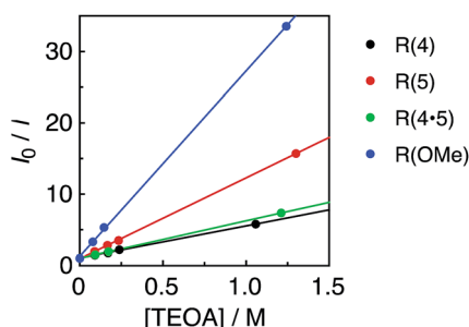
Fig. 3 Stern–Volmer plots obtained from the emission quenching of R(X) using TEOA in DMF under Ar; \lambda_{ex} = 400 nm.
