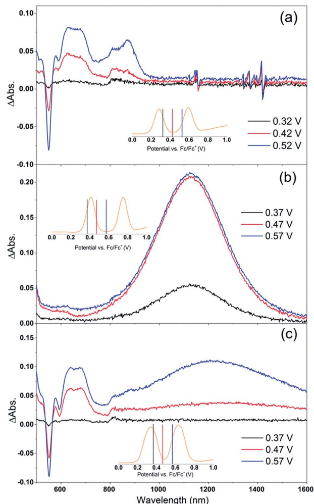
Fig. 4 Spectro-electrochemical (SEC) spectra of (a) Por, (b) Cb-TPA and (c) Por-(Cb-TPA) at different oxidation potentials vs. Fc/Fc + . For wavelength range from 230 nm, see Fig. S4.†
