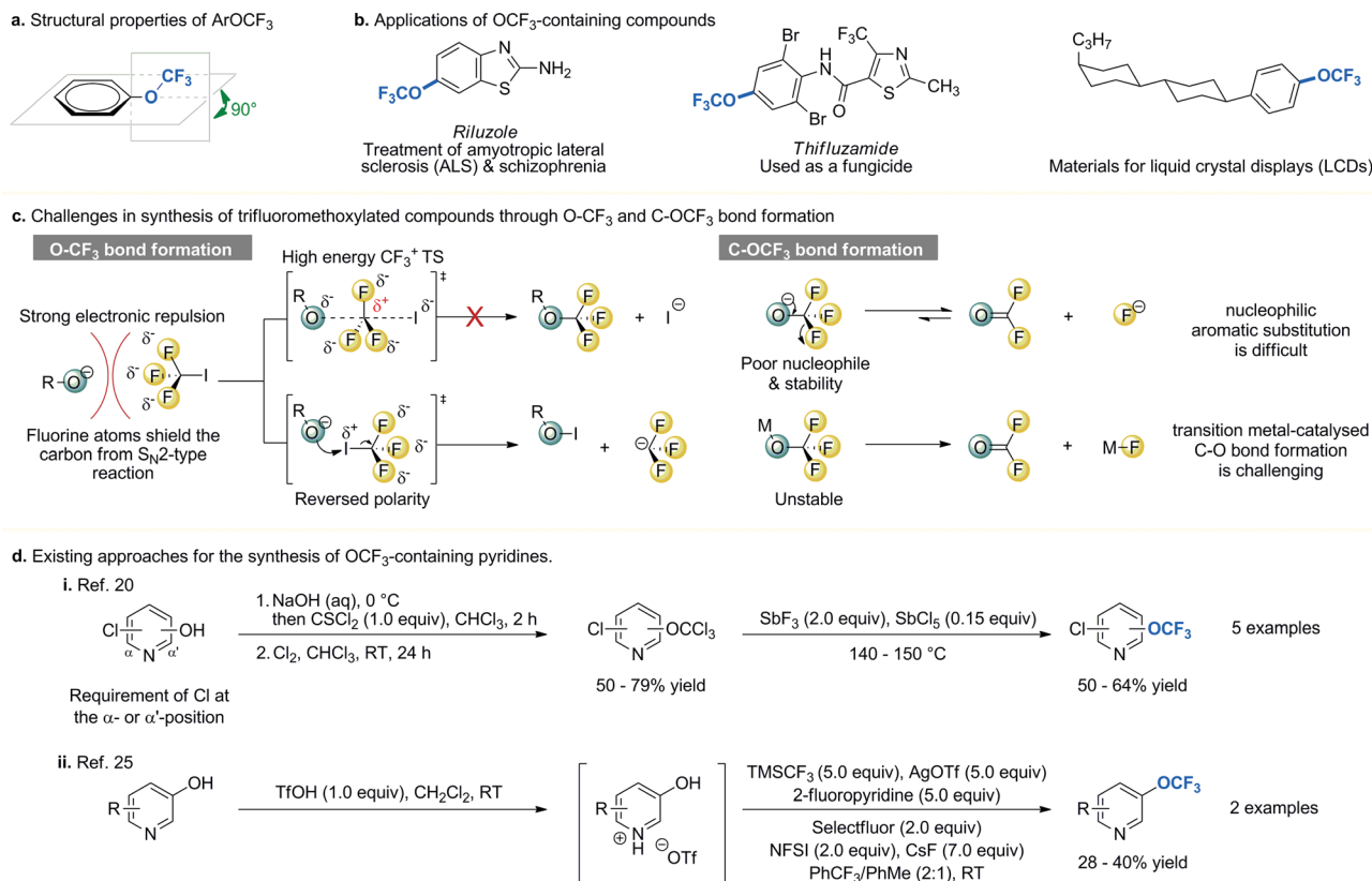
Fig. 1 Properties, applications, synthetic challenges and methods of synthesis of \text{OCF}_3 -containing compounds. NFSI = N -fluorobenzenesulfonimide, TMSCF 3 = trifluoromethyltrimethylsilane.
