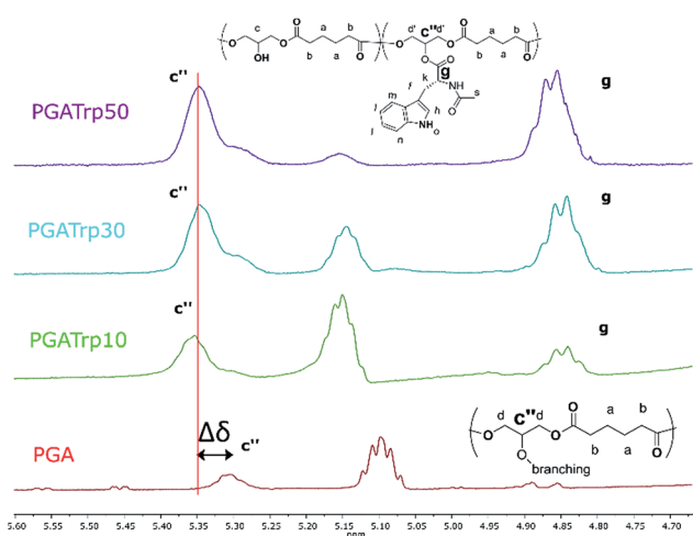
Fig. 1 ^1\text{H} NMR inset between 5.60 and 4.70 ppm of PGA and PGATrp10–30 and 50. Polymer backbone peak shifting ( c'' ) after coupling is highlighted. It is also possible to see that the trisubstituted PGA unit increases with Trp amount (g) supporting that functionalization has occurred.
