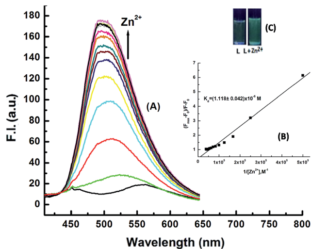
Fig. 4 (A) Fluorescence titration of H 3 SAL-NH (20 μM) in HEPES buffer at pH 7.2 recorded in THF : H 2 O (6 : 4, v/v) with the gradual addition Zn(NO 3 ) 2 · 6H 2 O with \lambda_{ex} = 398 nm and \lambda_{em} = 498 nm. (B) B–H plot of F.I. vs. 1/[Zn^{2+}] ; (C) UV-exposed emission image of H 3 SAL-NH with Zn 2+ .
