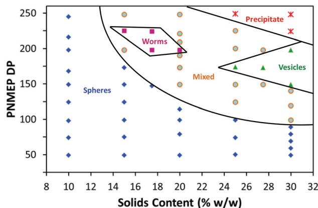
Fig. 5 Phase diagram for a series of PSMA 14 –PNMEPx diblock copolymers synthesised by RAFT dispersion polymerisation of NMEP in n -dodecane at various concentrations ranging between 10 and 30% w/w solids. Post-polymerisation analysis of each diblock copolymer dispersion by TEM determined the phase boundaries.
