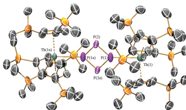
Fig. 1 Molecular structure of 1-C 7 H 8 with selected atom labelling and displacement ellipsoids set at 30% probability level. Th(1) and P(1) are on special positions, hence no equator quadratics could be generated. Hydrogen atoms, phosphorous and silyl group disorder components and lattice toluene have been removed for clarity. Symmetry operation to generate equivalent atoms: i = -x, -y, -z . Selected bond distances [Å] and angles [°]: Th(1)–P(1) 2.919(4), P(1)–P(2) 2.051(9), Th(1)–Cp centroid 2.543(5), Th(1)–P(1)–P(2) 133.0(2), P(1)–P(2)–P(1) 85.9(4), P(2)–P(1)–P(2) 94.1(4), Cp centroid ...Th(1)–Cp centroid 119.1(2).
