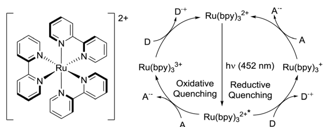
Fig. 1 Structure of [\text{Ru}(\text{bpy})_3]^{2+} and its oxidative and reductive quenching cycles.
