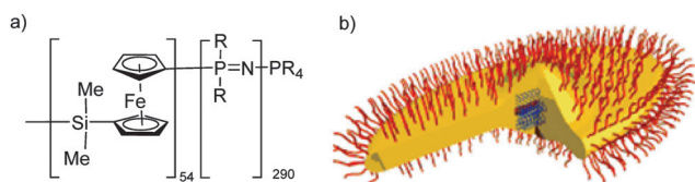
Fig. 14 Chemical structure of the block copolymer consisting of poly(ferrocenylsilane) and polyphosphazene ( R = OCH_2CF_3 ) blocks (a) and an idealized graphic representation of the pointed-oval-shaped micelles after crystallization-driven living self-assembly (b). Adapted with permission from A. Presa Soto et al. , Angew. Chem., Int. Ed. , 2010, 49 , 8220. Copyright 2010 Wiley-VCH. 33
